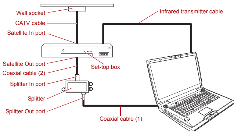
Figure 8-17 Connection method for the computer and set-top box
